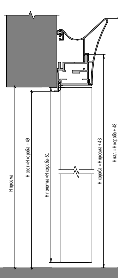
Открытие IN | IN Opening
