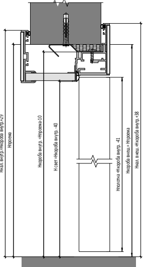
Открытие IN | IN Opening
