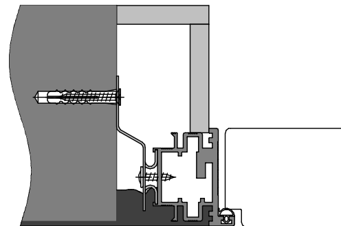
Открытие IN | IN Opening
