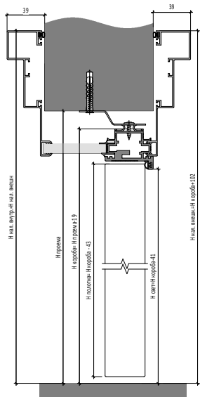
Открытие IN | IN Opening
