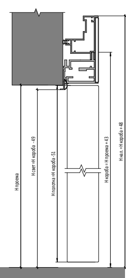
Открытие IN | IN Opening
