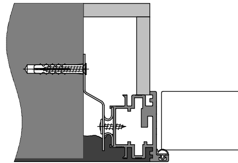
Открытие IN | IN Opening
