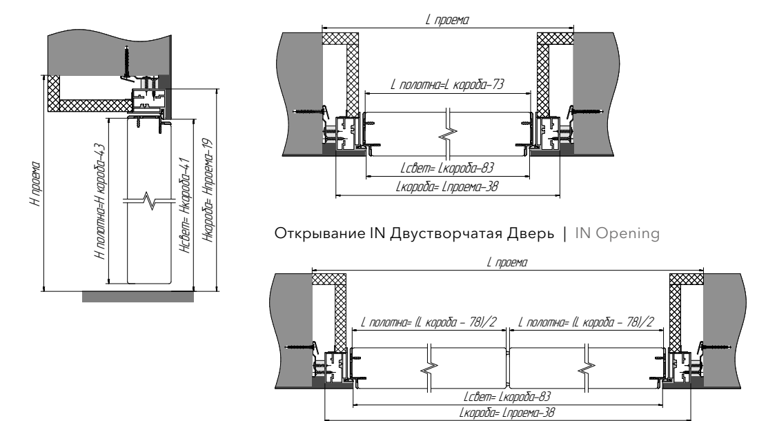
Открытие IN | IN Opening
