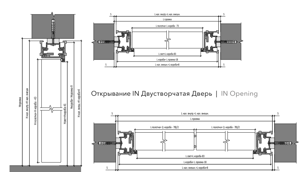
Открытие IN | IN Opening
